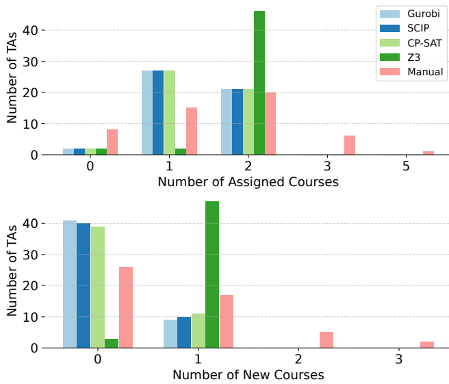
Fig. 2: Comparison of the number of assigned courses (upper) and number of new courses (lower) between solver output and manual teacher assignment for year 2022.
